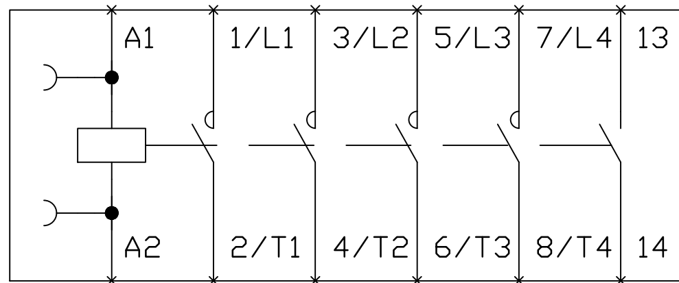
LEN00B004 Wiring Diagram
