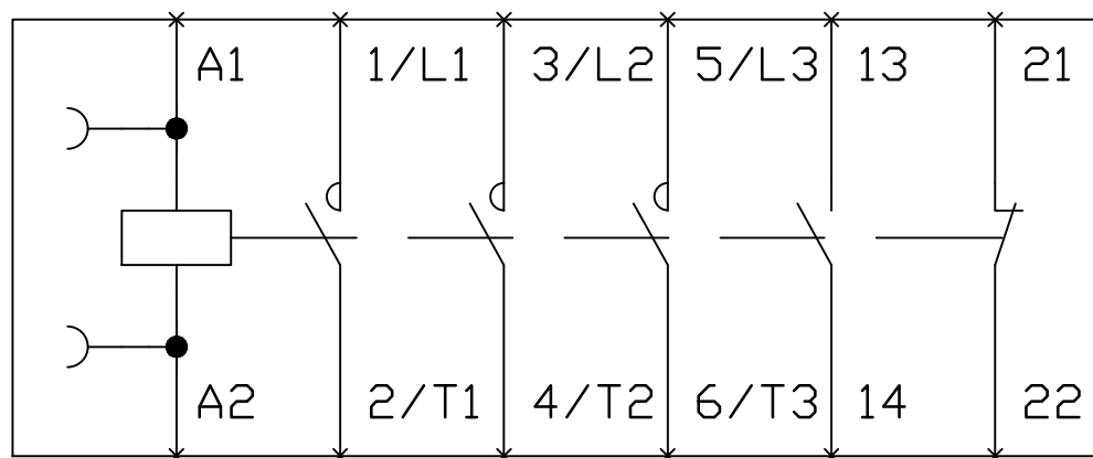
LEN00C003 Wiring Diagram
