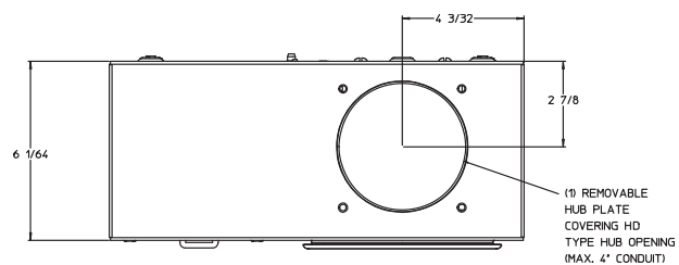
Top view for WP2211 and WEP2211
