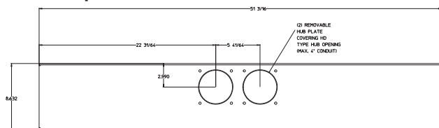
Top view for WEP6512 and WEP6612
