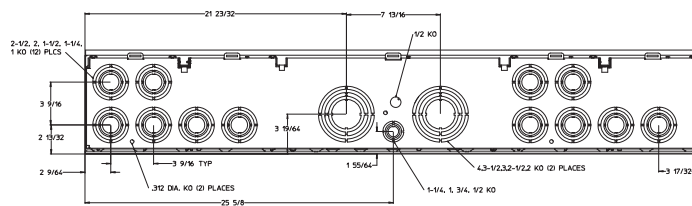
Bottom view for WEP6512 and WEP6612
